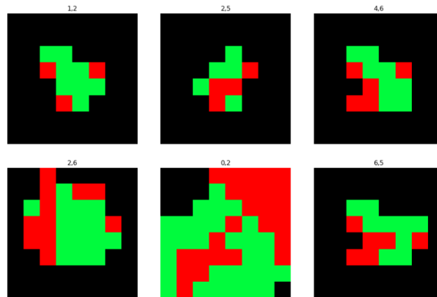
Fig. 3: Six example game boards with red denoting location of current player’s disks, green for opponent and black are unoccupied. Each board has as a title the game move predicted by the CNN.
