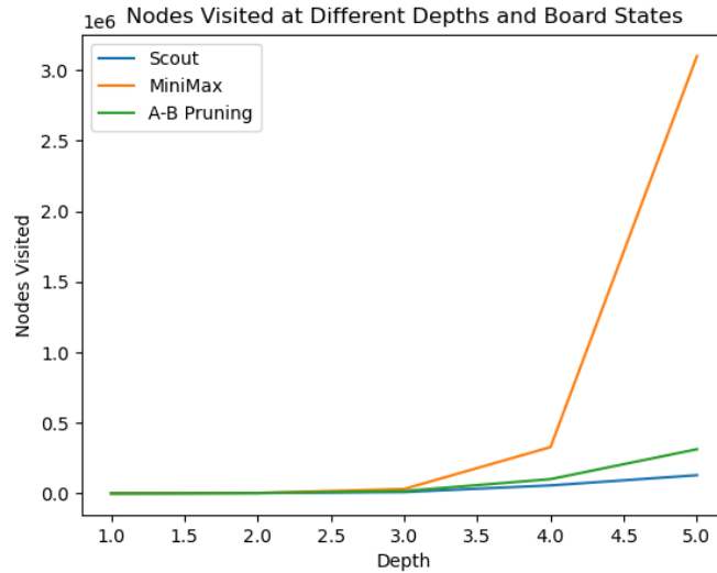
Fig. 5: Total Nodes Visited for a whole game, at random board states, depths and search Algorithms.
