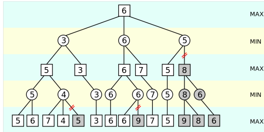
Fig. 2: A-B Pruning Example [9]
