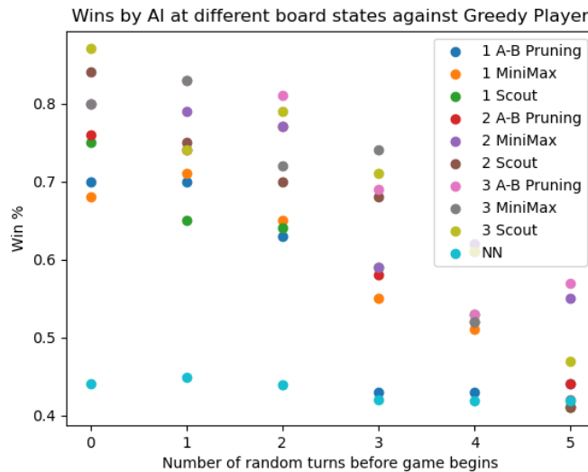
Fig. 4: Increasing depths resulted in more wins.
